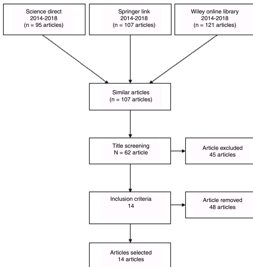
Figure 1 PRISMA diagram.
